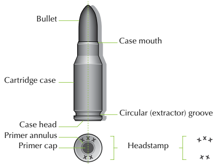
Figure 4 Components of a small-calibre cartridge
