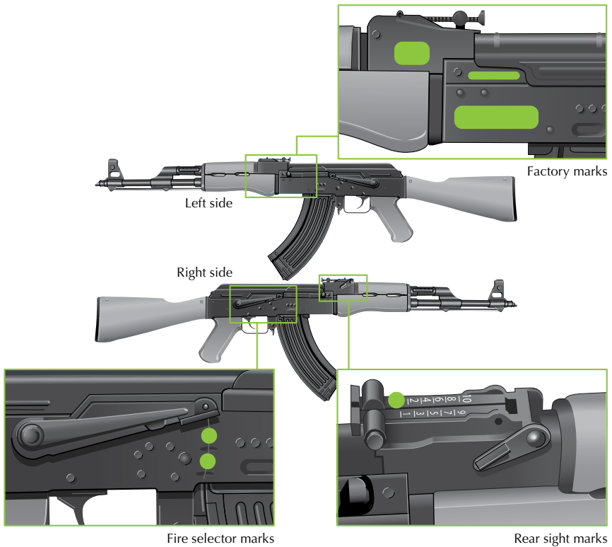
Figure 2 Positions of identifying marks on AK-pattern weapons
