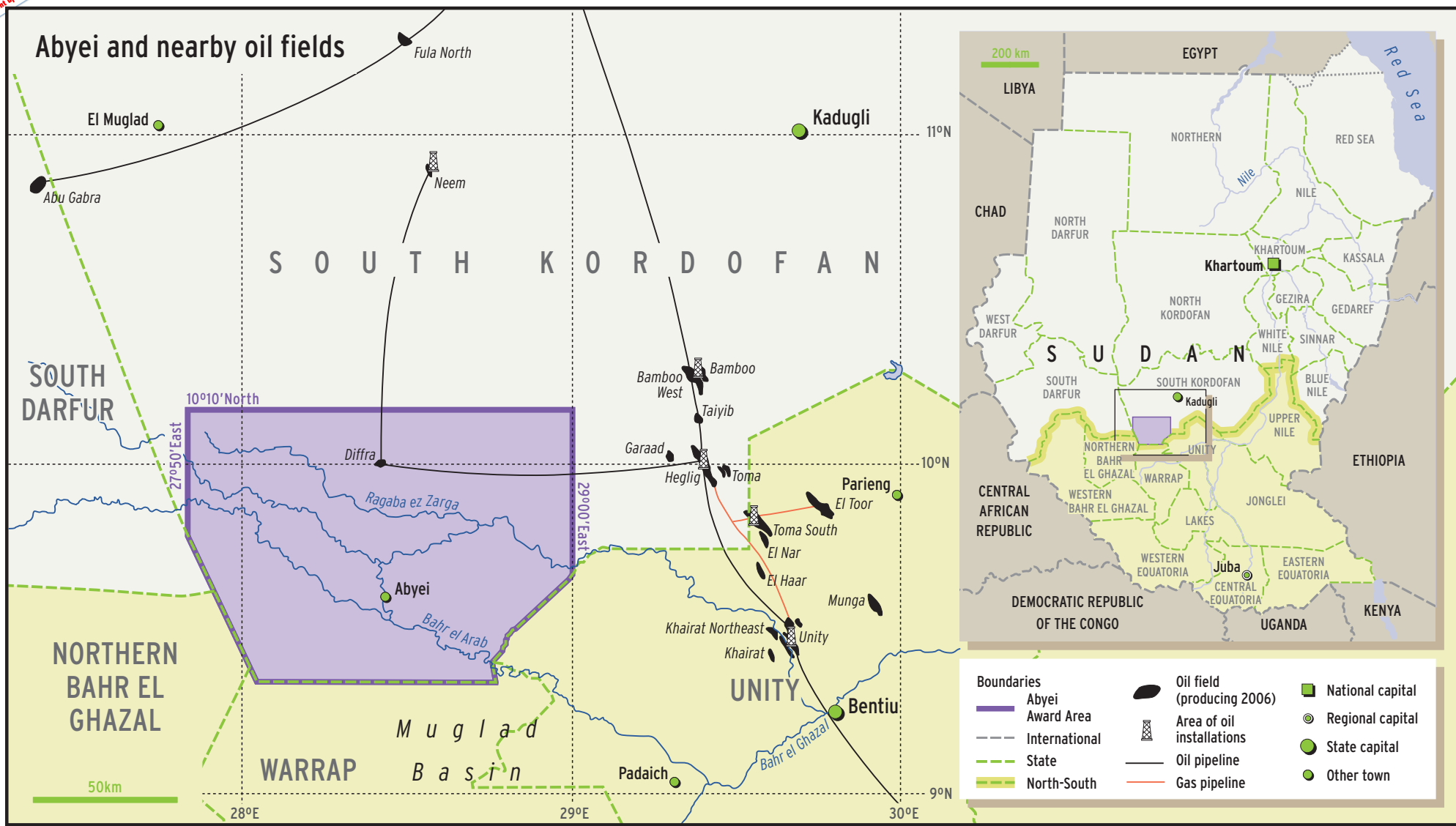
Abyei coordinates: as per the Abyei Arbitral Tribunal Source: Oil fields: IHS Energy, 2006
